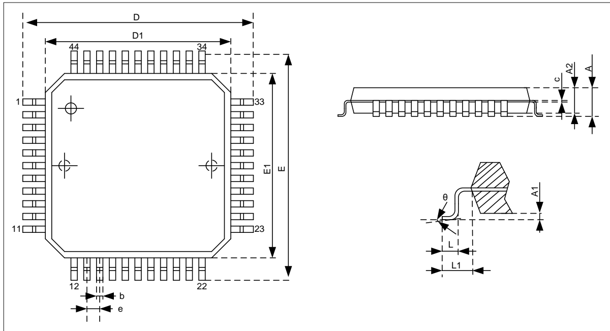
LQFP44
